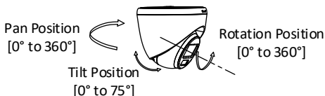
Figure 2-21 3-Axis Adjustment
