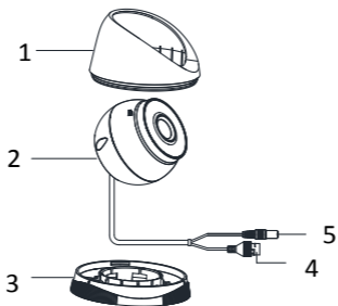
Figure 1-1 Type I Turret Camera Overview
