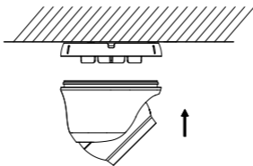
Figure 2-5 Install the Camera Body
